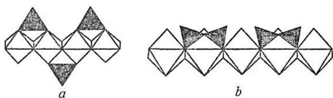
Fig. 13. Elementary-silicon-oxygen units of ortho-group \text{SiO}_4^{4-} in the structure of Mg-pyroxene enstatite ( a ) and diortho-group \text{Si}_2\text{O}_7^{6-} in Ca-pyroxene wollastonite ( b )
