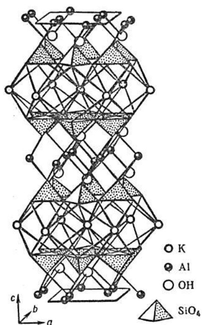
Fig. 17. A fragment (elementary packet) of the layered crystal structure of muscovite KAl_2(AlSi_3O_{10}XOH)_2 , illustrating the alternation of aluminum-silicon-oxygen layers of polyhedral meshes with the large aluminum and potassium cations, reminiscent of the DNA chain
